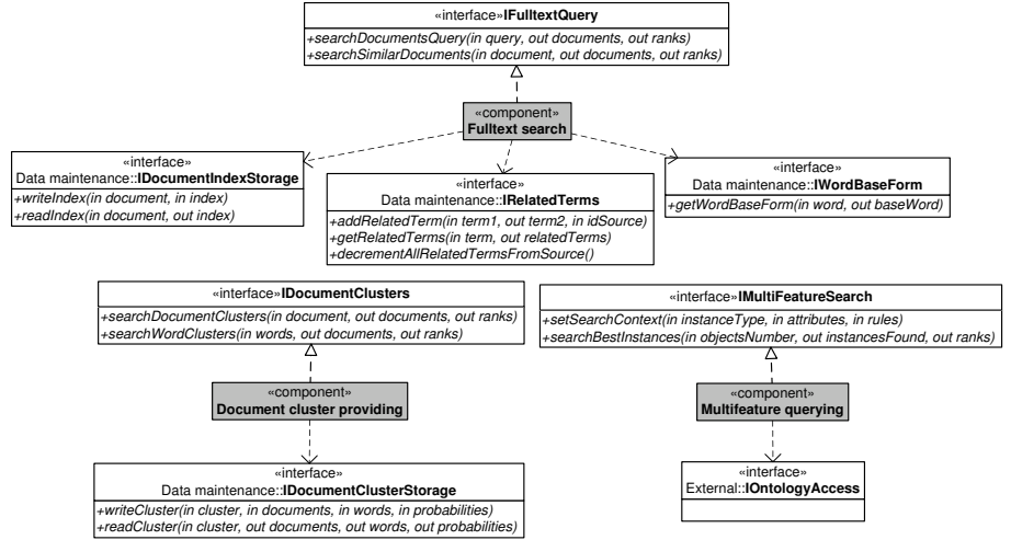
Fig. 9. The components that realize the functionality of the Data Search subsystem.
