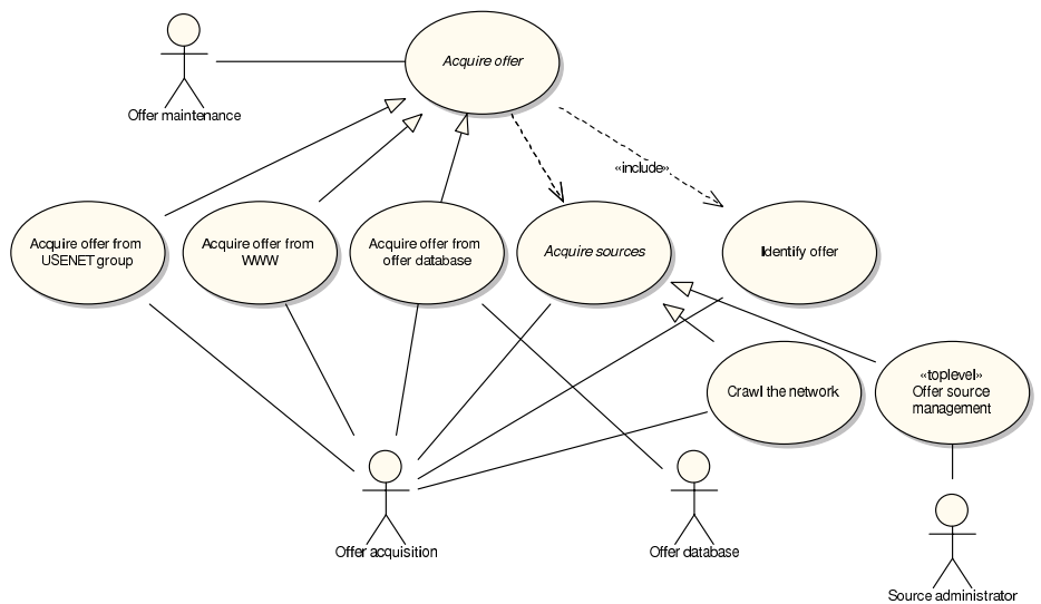
Fig. 7. Dealing with the different collaboration or different collaborating actors.
