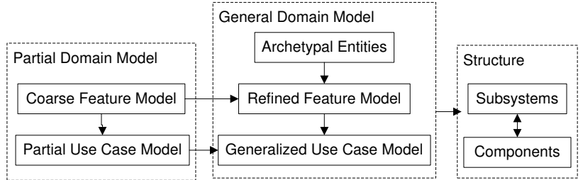
Fig. 1. Overview of the approach [10].
