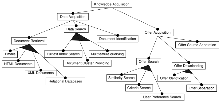
Fig. 5. Knowledge acquisition concept refinement.
