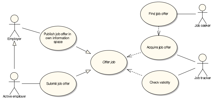
Fig. 3. A domain exploration level use case diagram.
