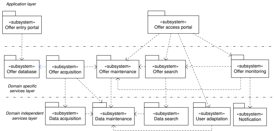
Fig. 8. The subsystem view.
